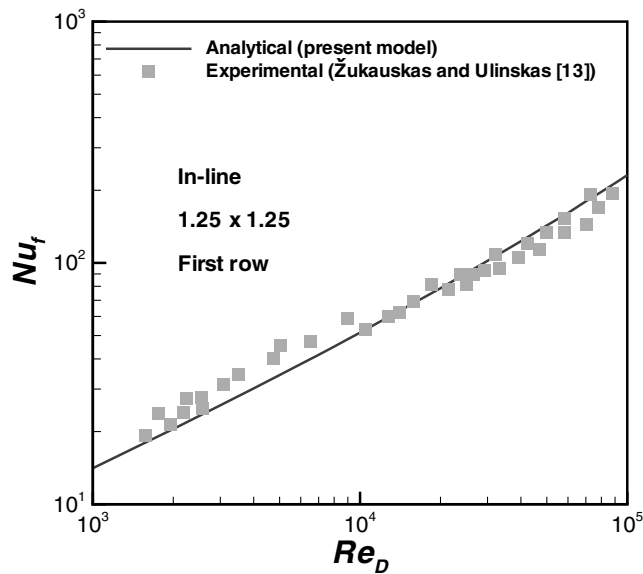
Fig. 4 Average heat transfer from the first row of a 1.25 \times 1.25 in-line tube bank.
