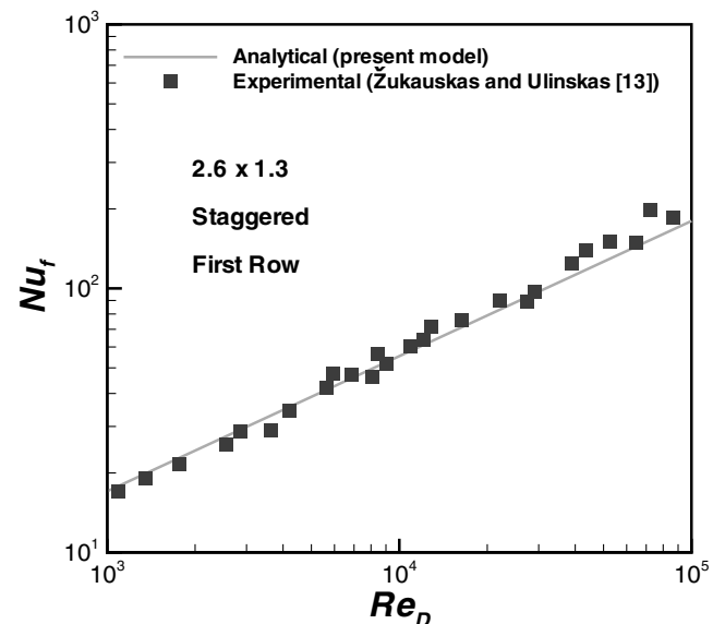
Fig. 7 Average heat transfer from the first row of a 2.6 \times 1.3 staggered tube bank.
