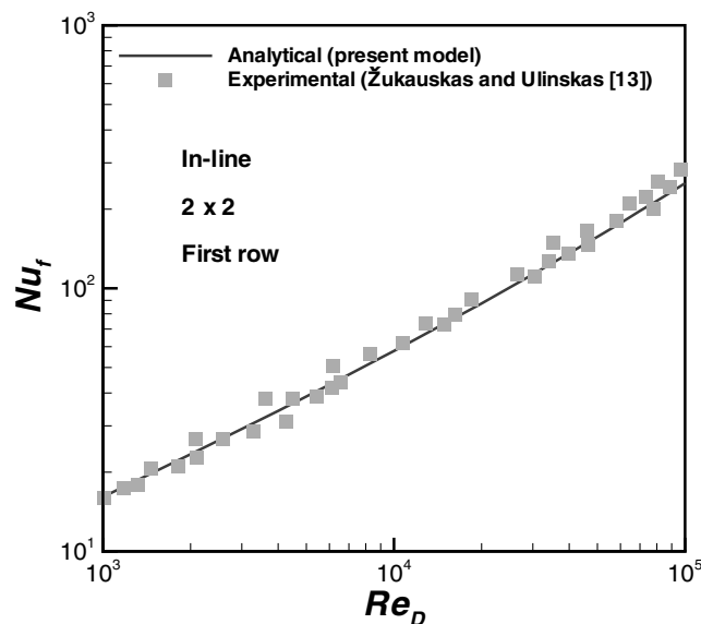
Fig. 5 Average heat transfer from the first row of a 2.0 \times 2.0 in-line tube bank.
