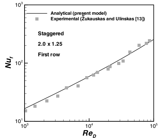
Fig. 6 Average heat transfer from the first row of a 2.0 \times 1.25 staggered tube bank.
